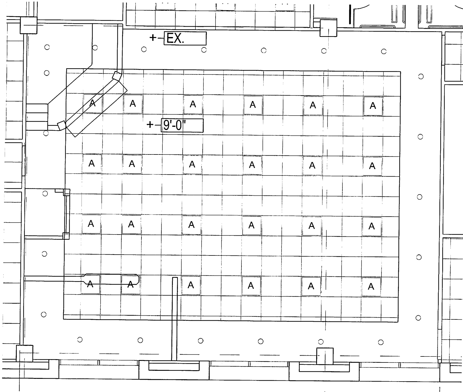
Burleson Sub-Courthouse JP Court Proposed Lighting Plan 03.24.2022
